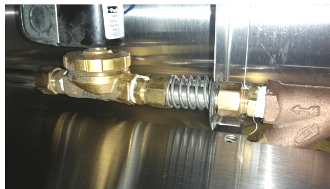
Showing 1/2" H 2 O solenoid, also stainless 1.5" drain tube
