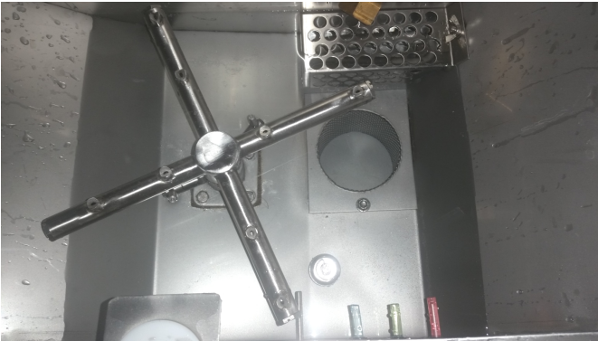
Wash tank with spray arm, float, secondary scrap screen
