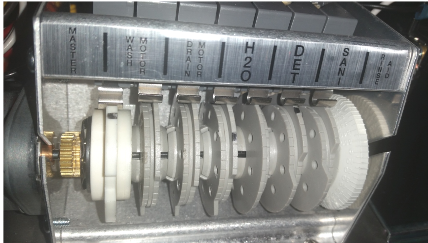
ASQ cam timer, fixed cams are MASTER, WASH MOTOR and DRAIN MOTOR
