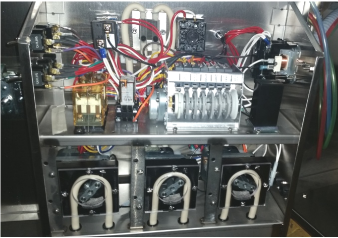
Showing deter, rinse, sanitizer internal chemical pumps
