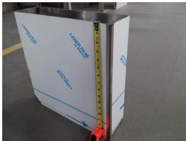
High 16" extension (285-6244) will fit into either the 4" opening or the 8" opening of the vent attachments. Thus making 74.25" or 78.25" possible in extensions from the floor.
