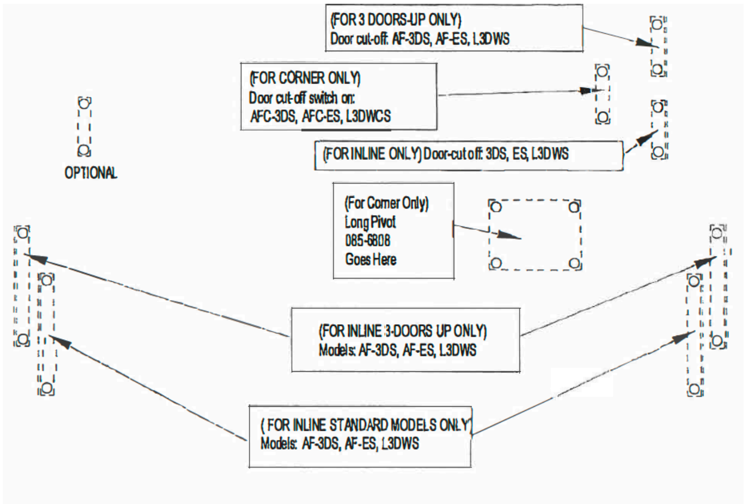
BACK PANEL OF HOOD FOR AF-3DS, AF-ES, L3DWS
