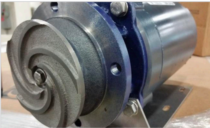
Open impeller (282-6308) 5 vane, 4.0" dia., low profile, screws on – right hand thread w/secure bolt (098-1443) washer (098-2413) Pump cover (282-6306), Rear housing (282-6307), Shaft Seal (292-2002), Fiber gasket (289-6609) Used on: ADC-44/66 for 1/3hp rinse pump w/motor 291-1003
