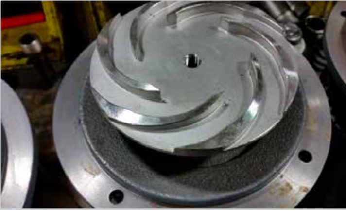
Open impeller (082-6312) 6 vanes modified, 5.0" dia., screws on – right hand thread Pump cover–stud mounted (082-6307), Rear housing (082-6301), Shaft Seal (092-2001), O-ring gasket (089-6309) Used on: AF-ES & AFC-ES 1.5hp pump w/motor 091-1001 and 5AGES 1.0hp pump w/motor 091-1024
