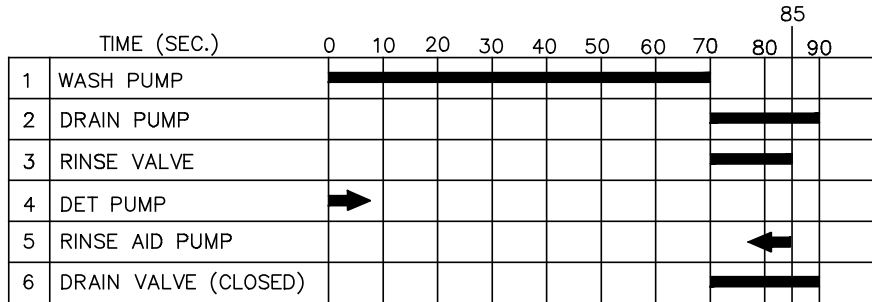
TIMING CHART FOR FRESH WATER RINSE EXTENDED WASH ADDS 15 MINUTES EXTRA WASHING TIME AT 70 SECS SWITCH MAY BE PUSHED ANY TIME FROM 0.5 TO 70 SEC
