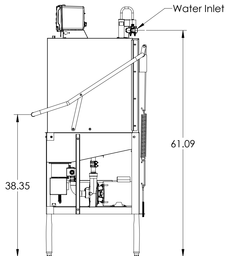
SIDE VIEW
